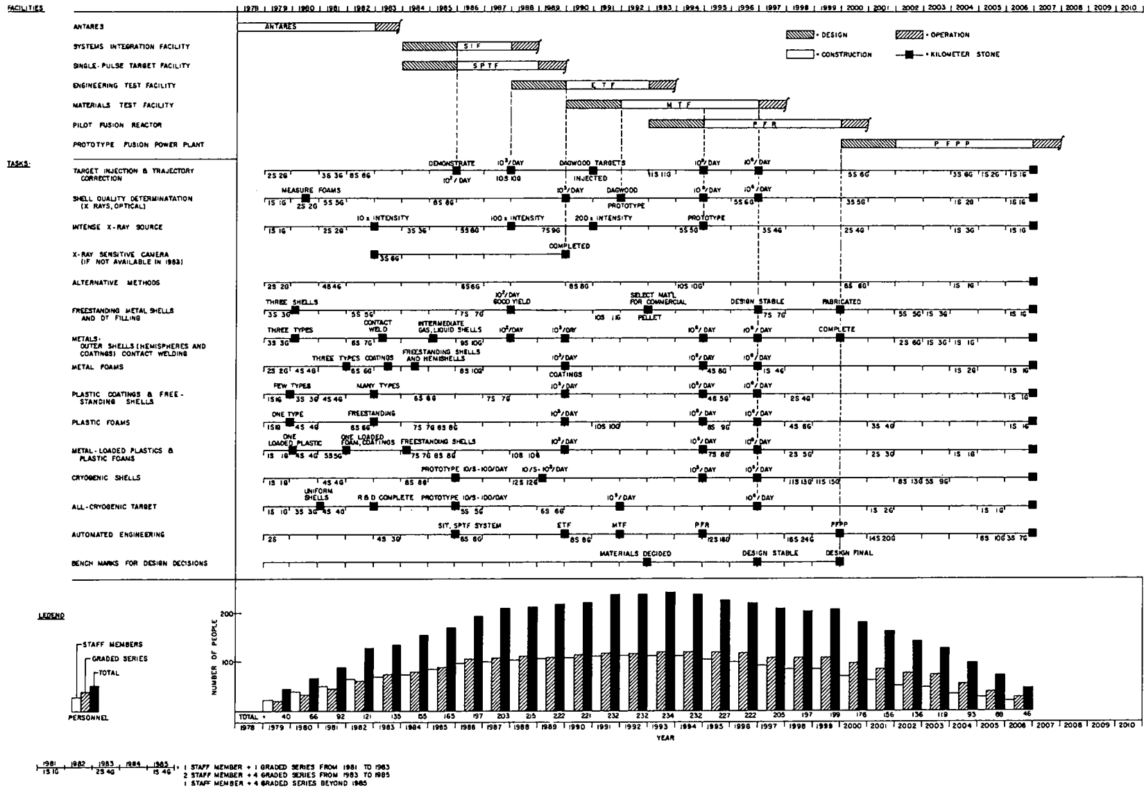
Fig. 6. Personnel requirements by task for the Advanced Laser Fusion Target Research and Development Program.
