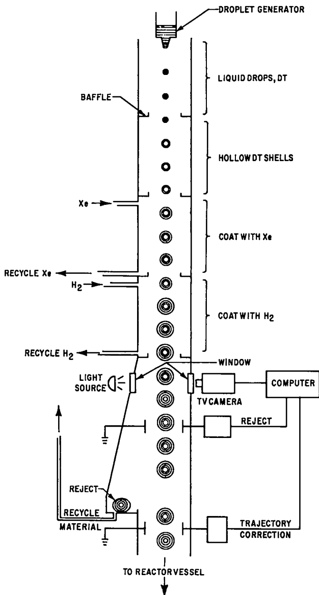
Fig. 5. Drop tower for making special cryogenic targets.
