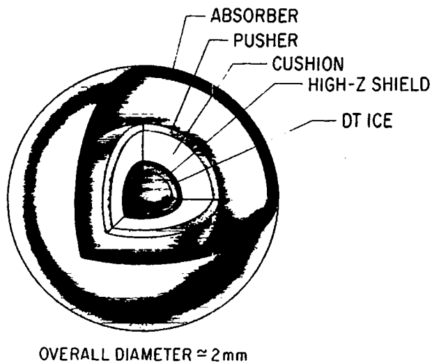
Fig. 2. Example of a Dagwood target with six shells.
