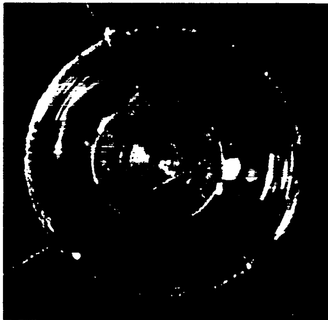
Fig. 3. Six-shell target for Helios. One gold and one plastic hemishell have been removed to show the construction and the DT-filled glass microballoon in the center. Beginning from the center, the shells are: (1) DT ice, (2) glass, (3) vacuum, (4) gold, (5) vacuum, and (6) plastic. The diameter of the largest shell is 0.5 mm.
