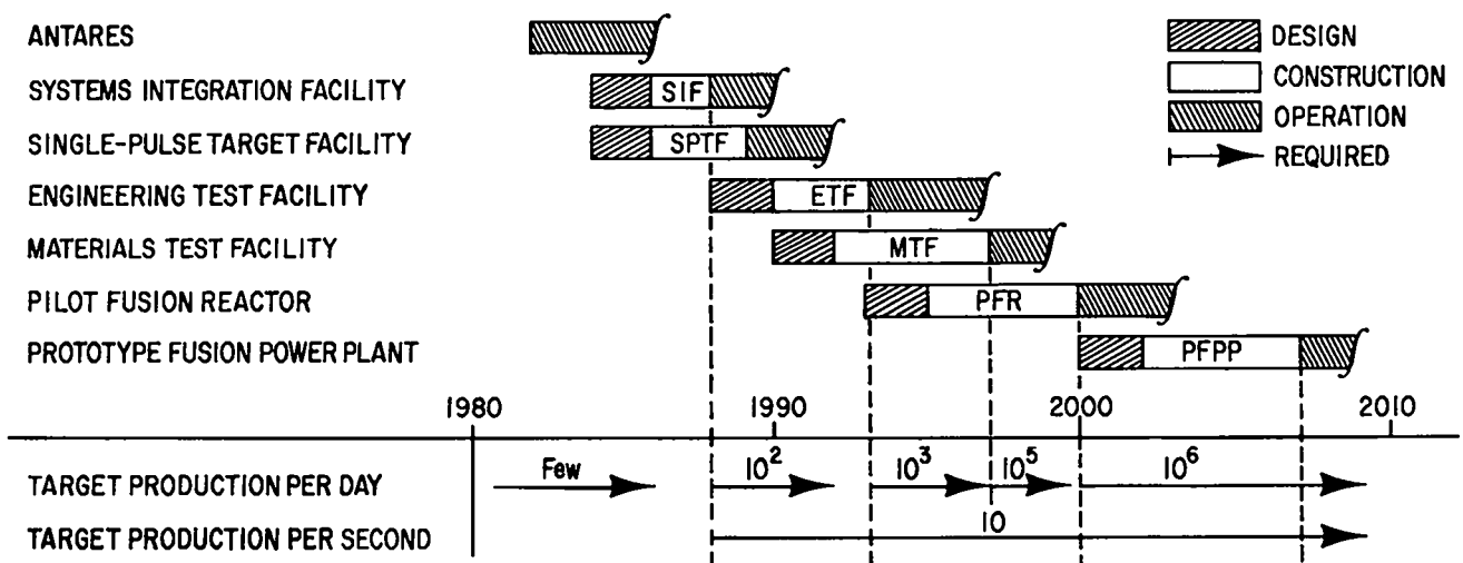
Fig. 1. Requirements for the Advanced Laser Fusion Target Research and Development Program. The time schedule for the facilities outlined in Ref. 1 is shown with the pellet production rates for each facility.
