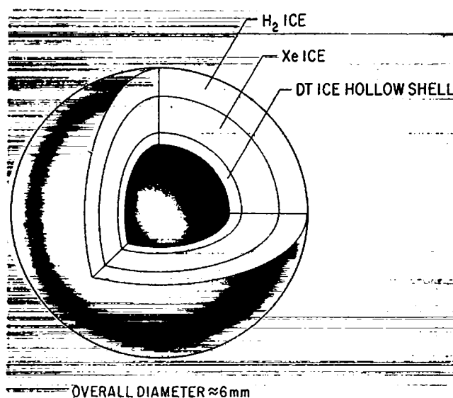
Fig. 4. All-cryogenic target with three layers.
